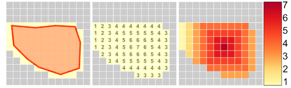
Figure 3: The mapping of a shape (left) to numbers (middle) to colors (right) determining the off-screen grid cell color.
